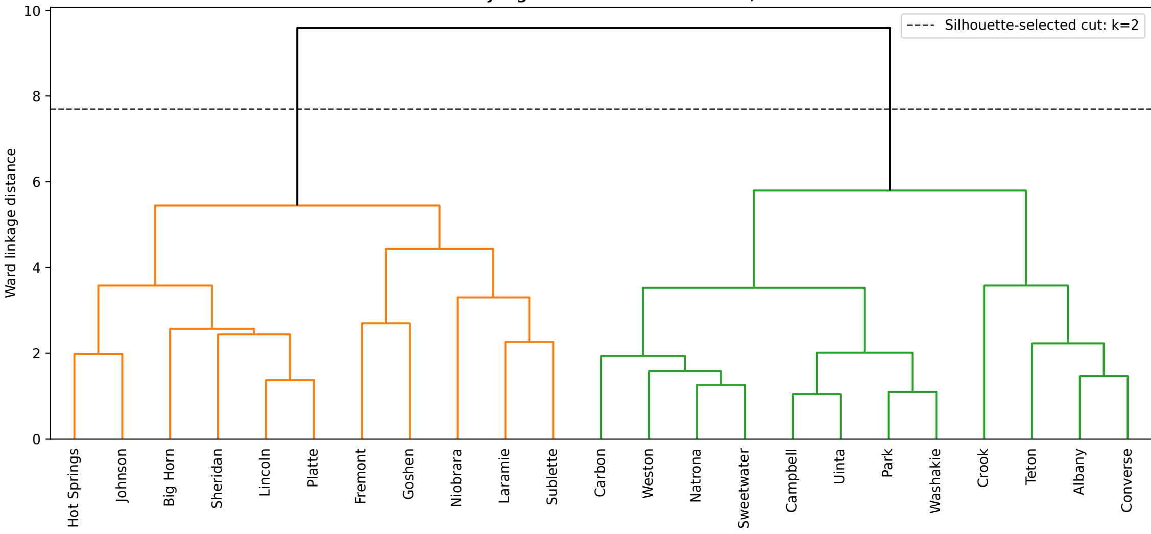
Ward Dendrogram — Simplified 6-Feature Space, 35-day Sakoe-Chiba Band Branch colors forced by highest silhouette score: k=2, silhouette=0.275
